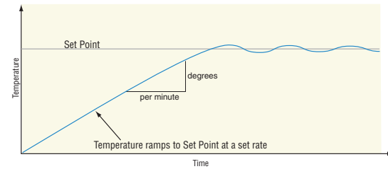
Heating System with Ramping
