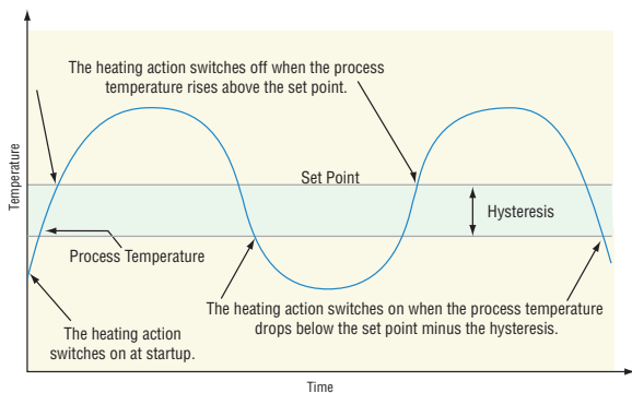
On/Off System Cycles
