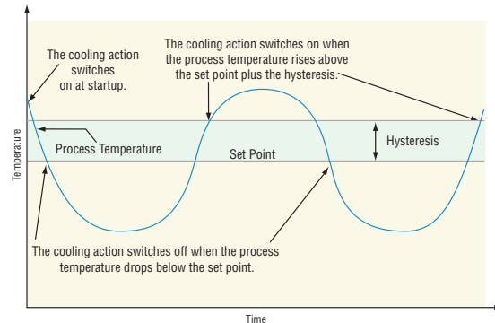
On/Off System Cycles
